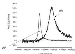
Frequency shift of the resonator while solid particles impact the surface
